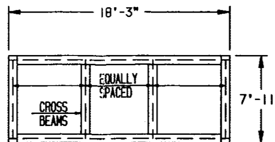
TYPICAL PLAN OF SUPPORT SIZE OF BEAMS ACCORDING TO OPERATING WEIGHT OF UNIT.
